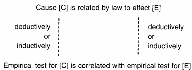
Figure 1.3 A Causal Theory Square
